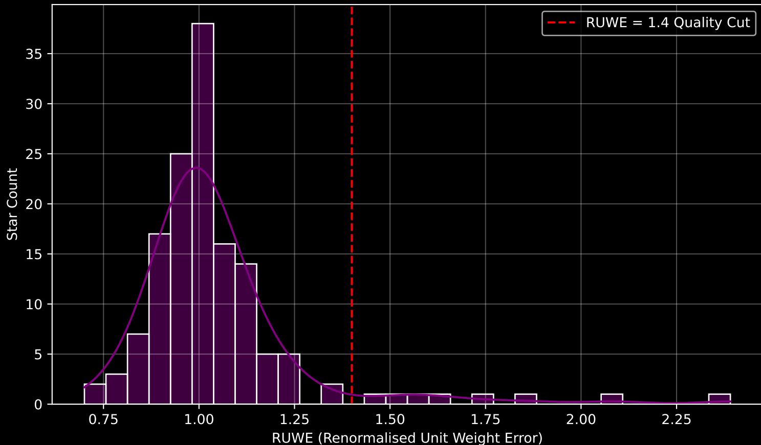
GAPOGEE DR17 Field [022-02] RUWE Distribution (n= 142)
