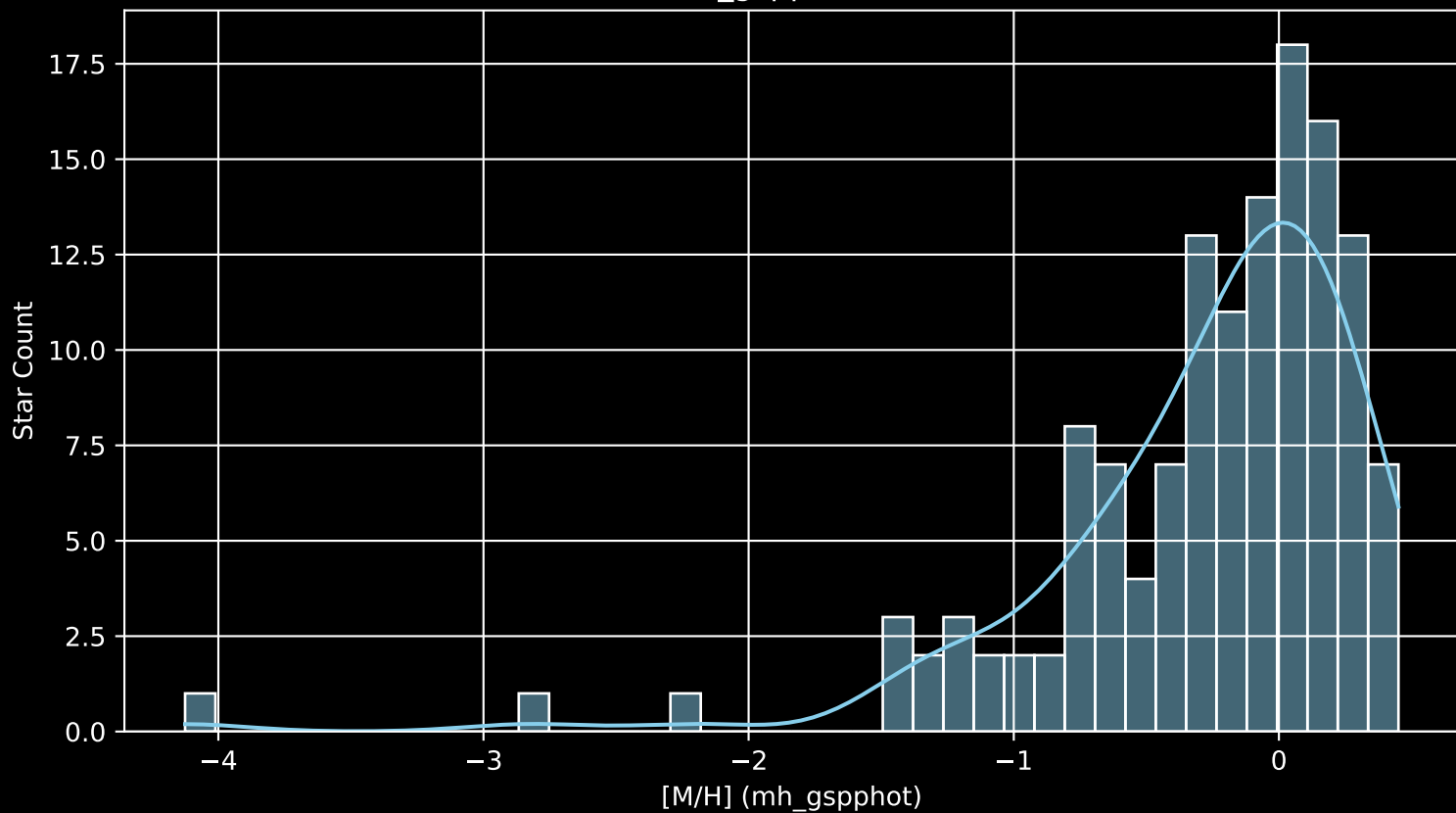
APOGEE DR17 Field: [022-02 [M/H] (mh_gspphot) (n= 135)
