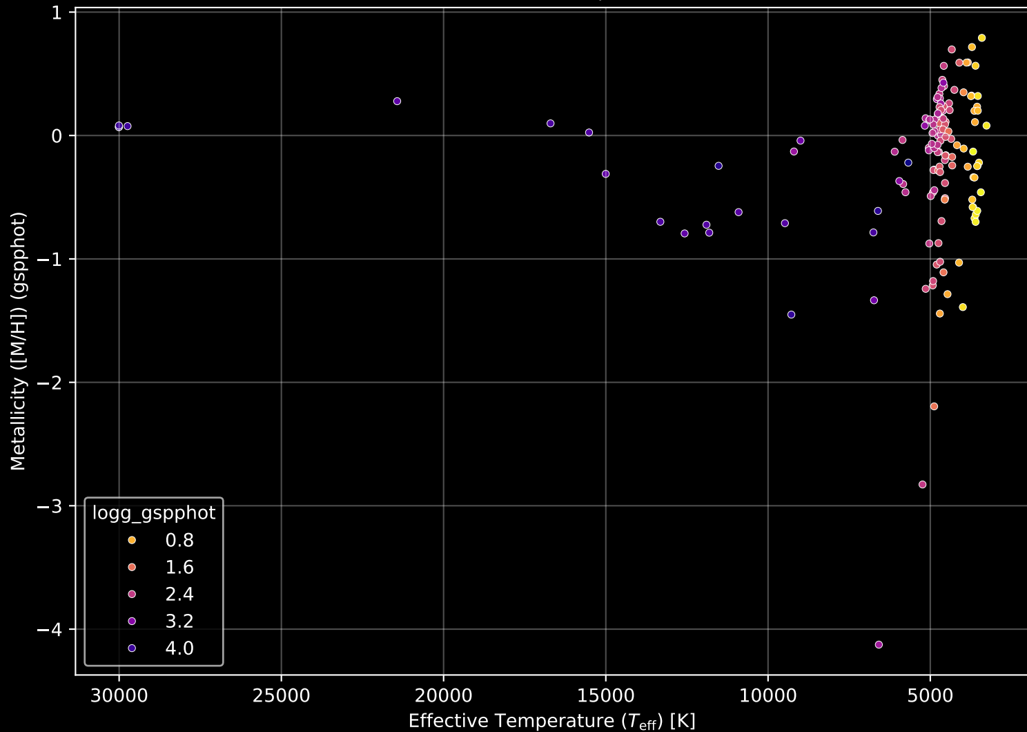
APOGEE DR17 Field: [022-02] Stellar Population Parameters (n= 143)
