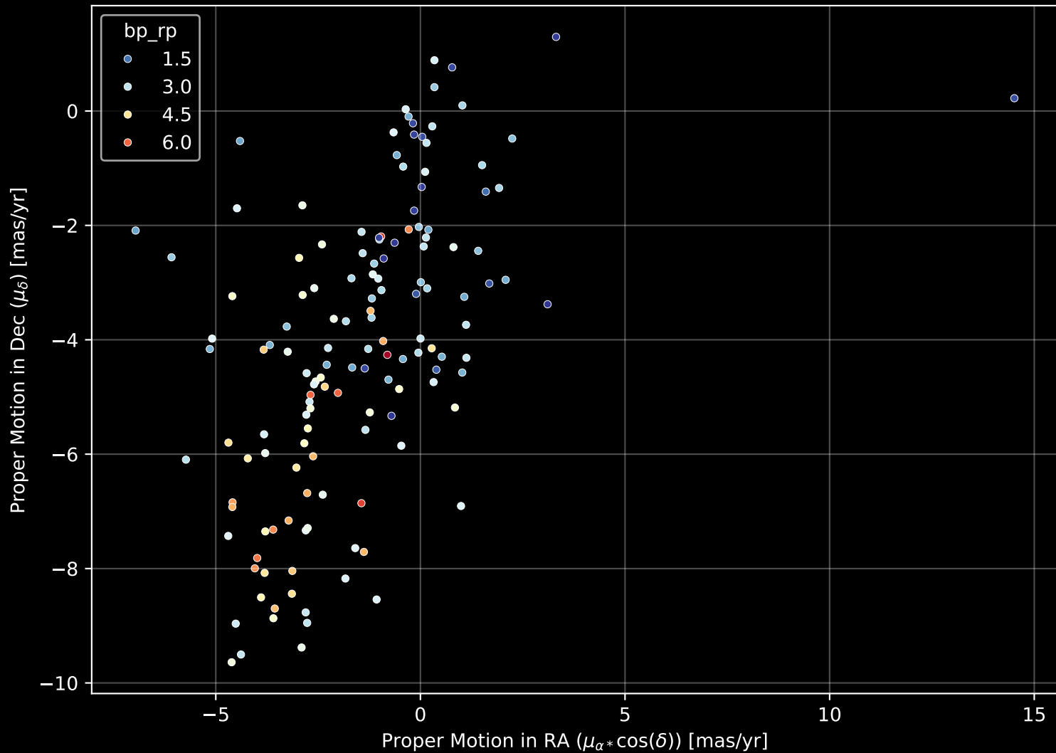
APOGEE DR17 Field: [022-02] Proper Motion Diagram (n= 143)
