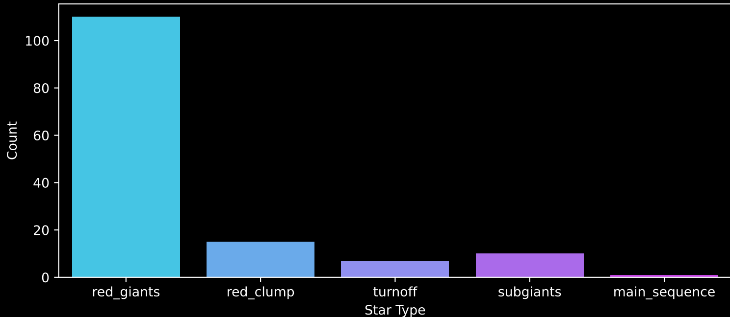
APOGEE DR17 Field: [022-02] Count plot of Star Type
