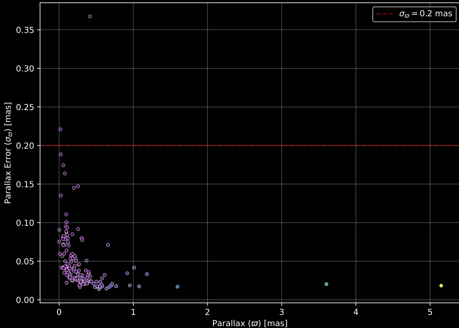
APOGEE DR17 Field: [022-02] Parallax Quality (n= 143)
